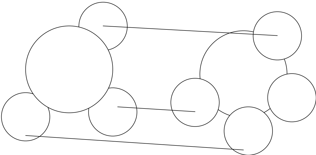
Figure 4. In this diagram the large circles again represent two fields and the smaller circles represent branches of these fields. The lines joining them represent work linking hitherto different branches. These lines thicken as the amount of articles and other research activities increase and thus become a new means of tracing the growth of an emerging field.
